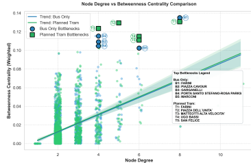
Figure 4: Degree vs betweenness centrality (jitter applied).
