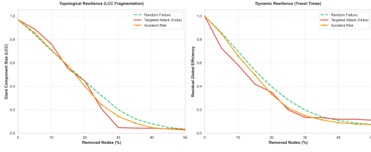
Figure 6: Operative stress: percolation curves (Left: size, Right: efficiency).
