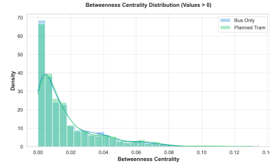
Figure 5: Betweenness distribution (values > 0) with a KDE curve.
